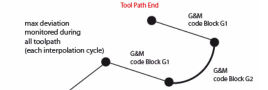
simple toolpath trajectory (composite segment for example)
