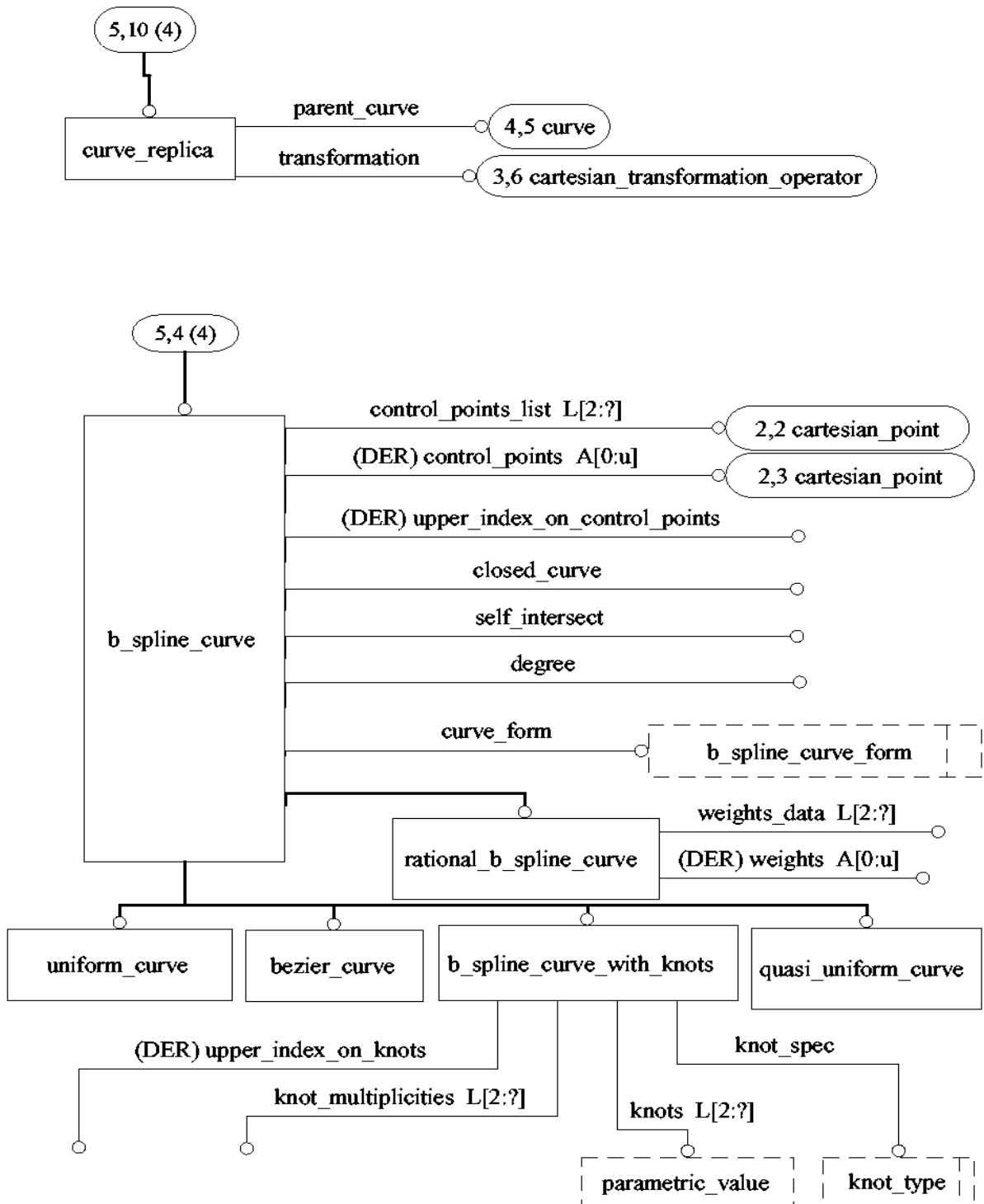
Figure C.5 - aic_geometrically_bounded_wireframe - EXPRESS-G diagram 5 of 6
