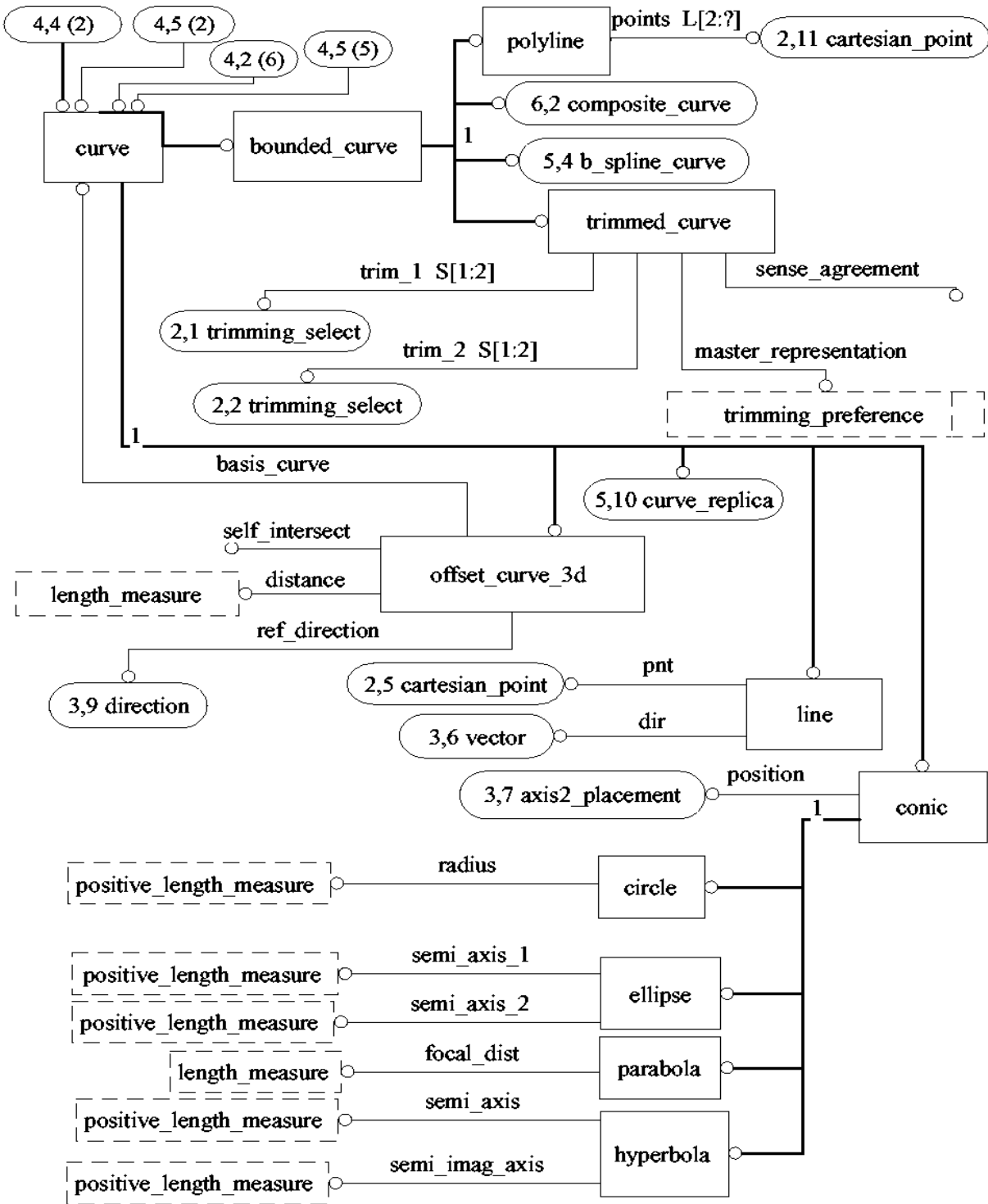
Figure C.4 - aic_geometrically_bounded_wireframe - EXPRESS-G diagram 4 of 6
